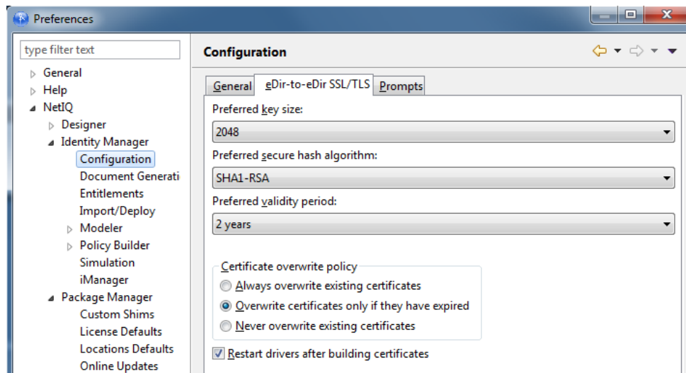
Figure 19-3 The Advanced TLS Configuration Dialog Box
